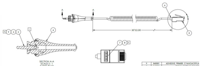
124330 CABLE, QR REPLACEMENT, TAT-5000S-RS232-QR
