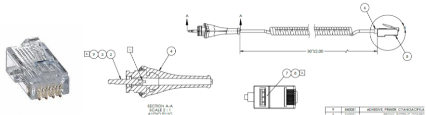
124330 CABLE, QR REPLACEMENT, TAT-5000S-RS232-QR
