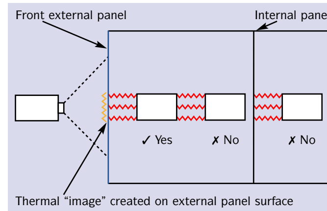
Thermal imaging can only provide a “snapshot” image from the outside.
